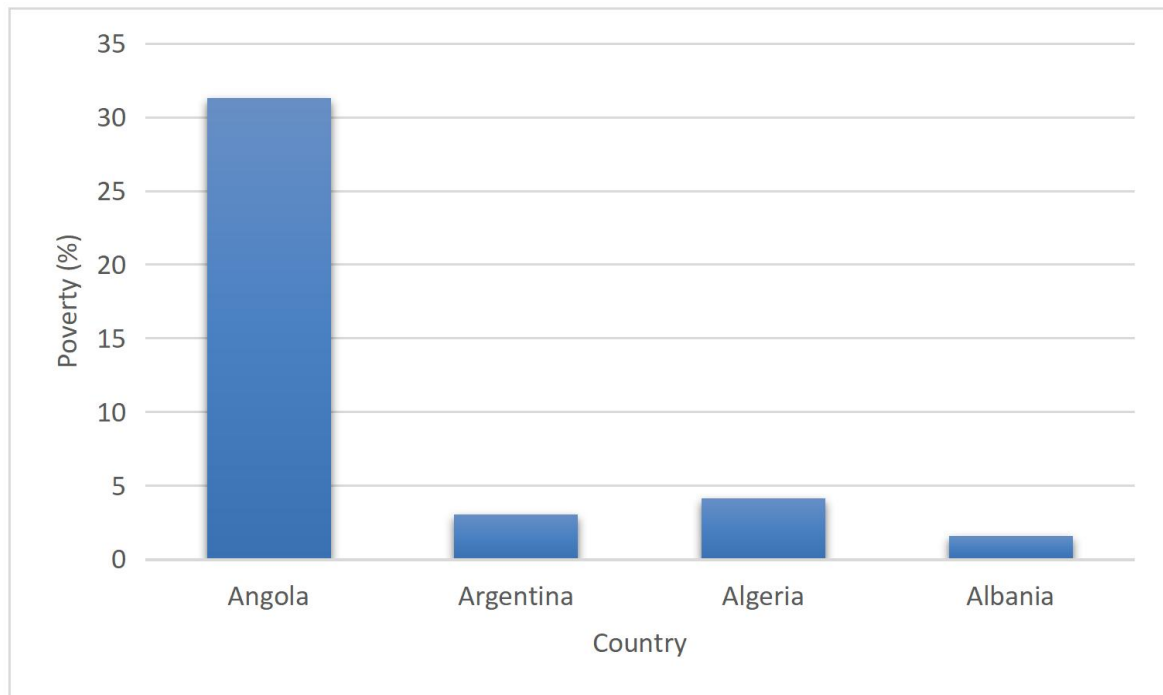
Figure 2. Poverty Levels Across Selected Countries
