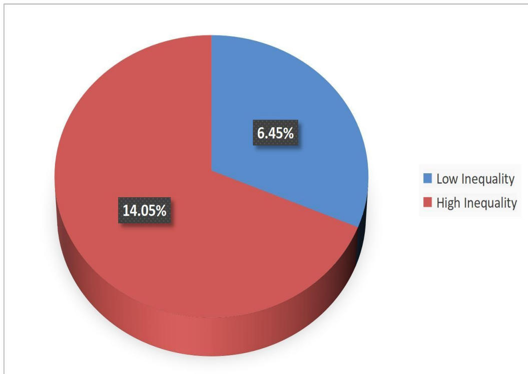
Figure 3. Poverty Distribution by Inequality Groups
